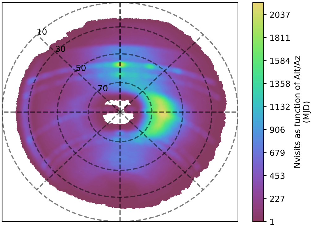
ddf_loaded_half_fl8_v3.4_10yrs r band: Nvisits as function of Alt/Az
