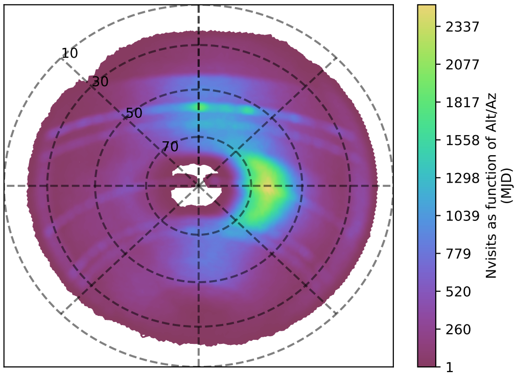
ddf_loaded_half_fl8_v3.4_10yrs i band: Nvisits as function of Alt/Az
