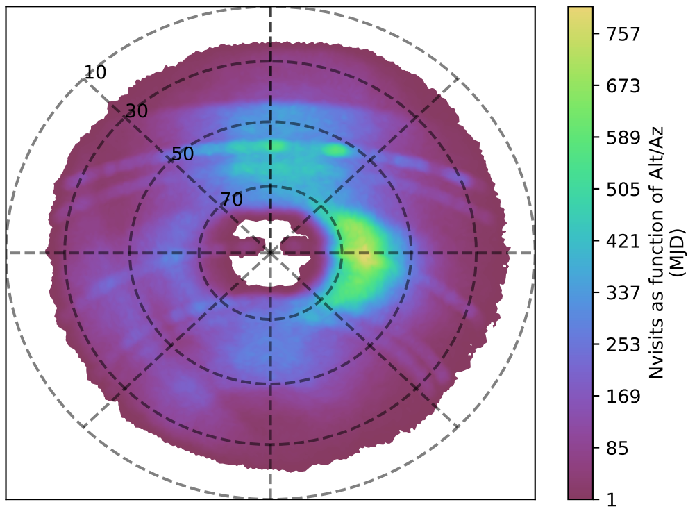
ddf_loaded_half_fl8_v3.4_10yrs g band: Nvisits as function of Alt/Az
