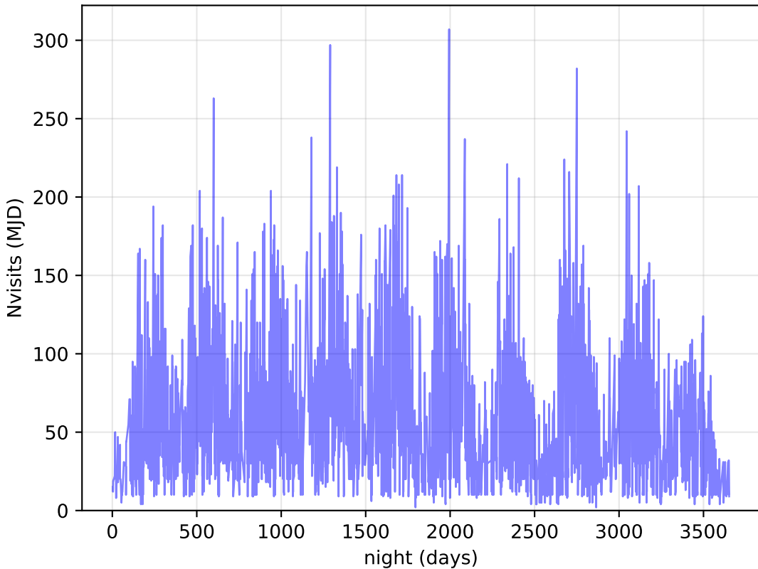
ddf_loaded_half_fl8_v3.4_10yrs DDF: Nvisits
