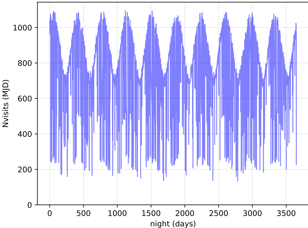
ddf_loaded_half_fl8_v3.4_10yrs All visits: Nvisits
