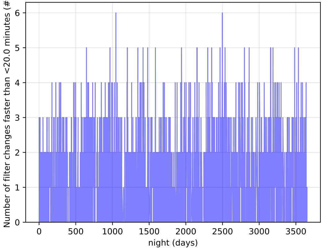
ddf_loaded_half_fl8_v3.4_10yrs Per Night: Number of filter changes faster than <20.0 minutes
