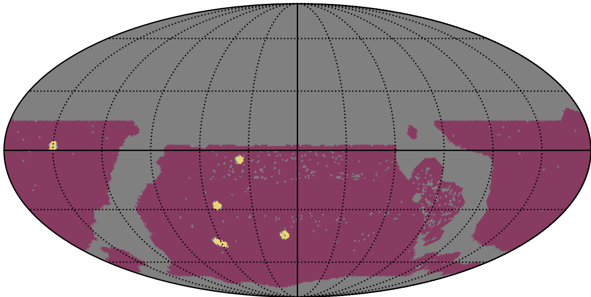
ddf_loaded_half_fl8_v3.4_10yrs WFD: NumberOfQuickRevisits
