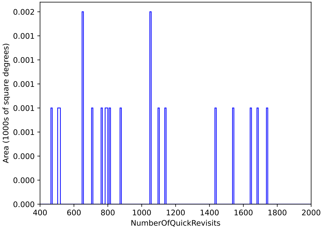
ddf_loaded_half_fl8_v3.4_10yrs WFD: NumberOfQuickRevisits
