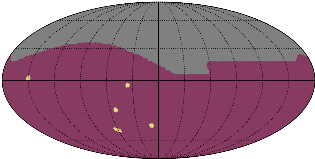
ddf_loaded_half_fl8_v3.4_10yrs All sky: NumberOfQuickRevisits
