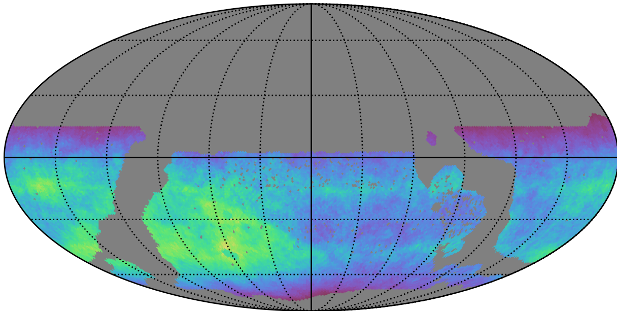
ddf_loaded_half_fl8_v3.4_10yrs WFD z band: Normalized Teff
