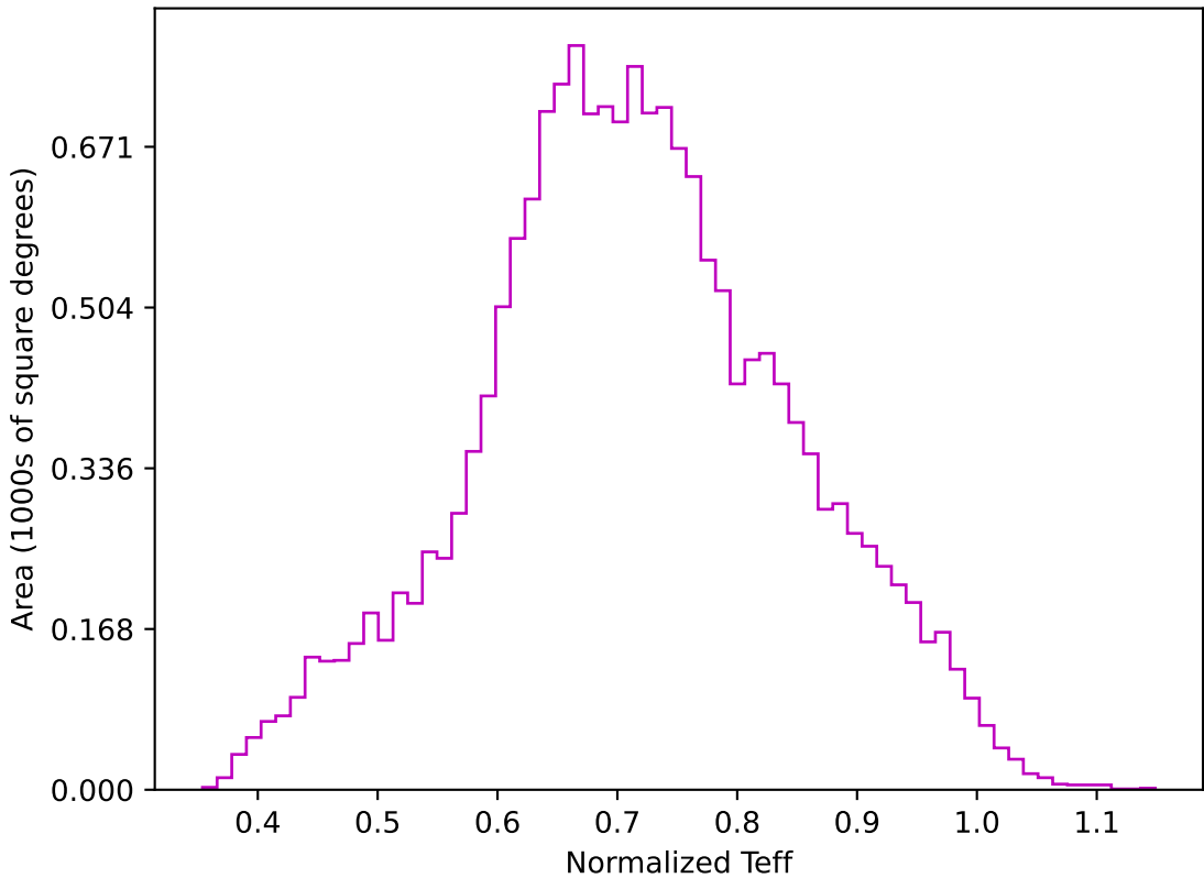
ddf_loaded_half_fl8_v3.4_10yrs WFD z band: Normalized Teff
