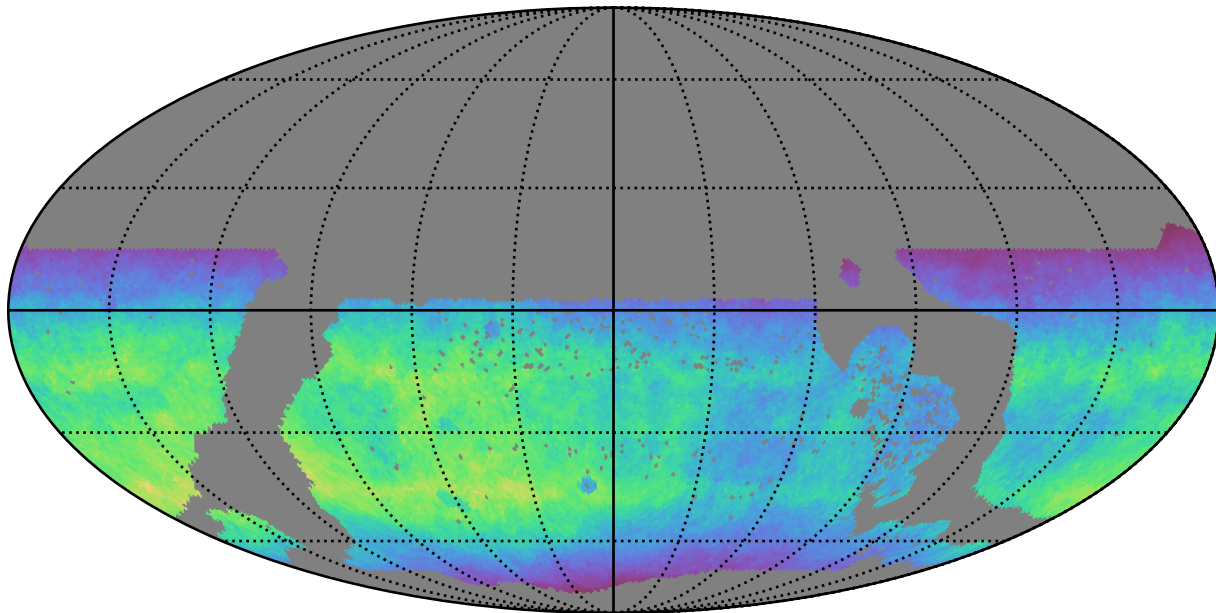
ddf_loaded_half_fl8_v3.4_10yrs WFD y band: Normalized Teff
