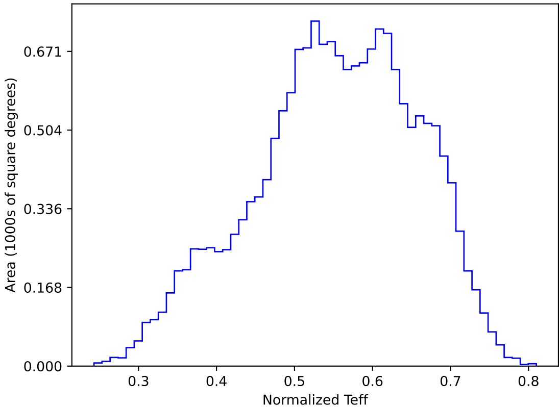
ddf_loaded_half_fl8_v3.4_10yrs WFD y band: Normalized Teff
