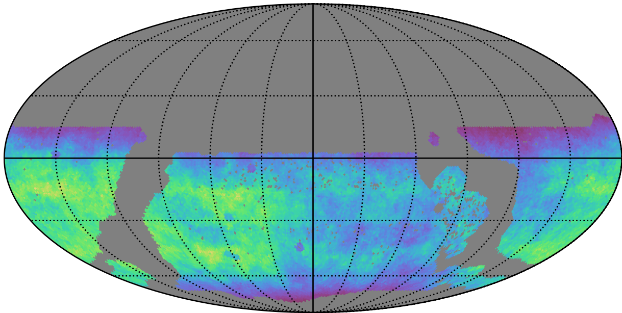
ddf_loaded_half_fl8_v3.4_10yrs WFD u band: Normalized Teff
