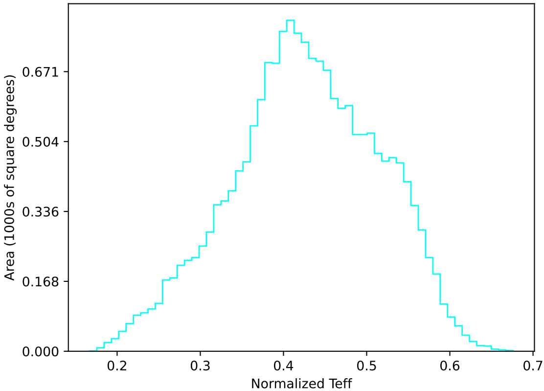
ddf_loaded_half_fl8_v3.4_10yrs WFD u band: Normalized Teff
