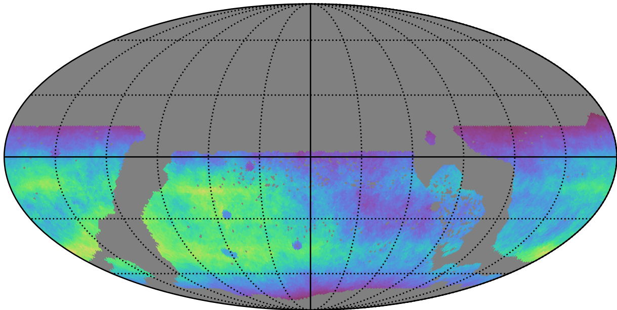
ddf_loaded_half_fl8_v3.4_10yrs WFD r band: Normalized Teff
