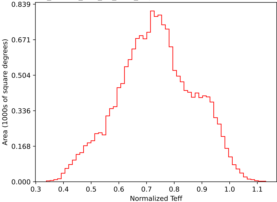
ddf_loaded_half_fl8_v3.4_10yrs WFD i band: Normalized Teff
