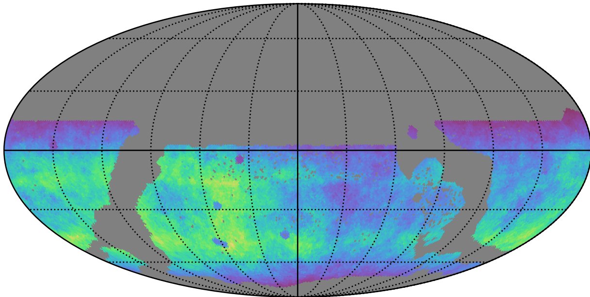
ddf_loaded_half_fl8_v3.4_10yrs WFD g band: Normalized Teff
