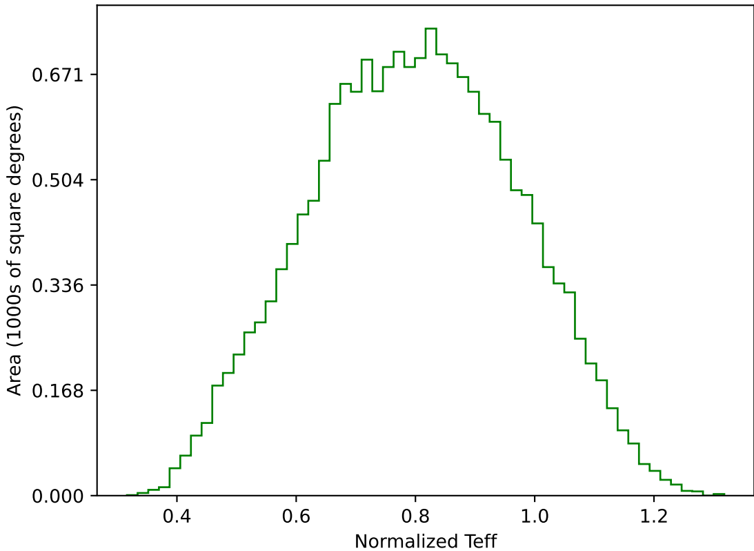
ddf_loaded_half_fl8_v3.4_10yrs WFD g band: Normalized Teff
