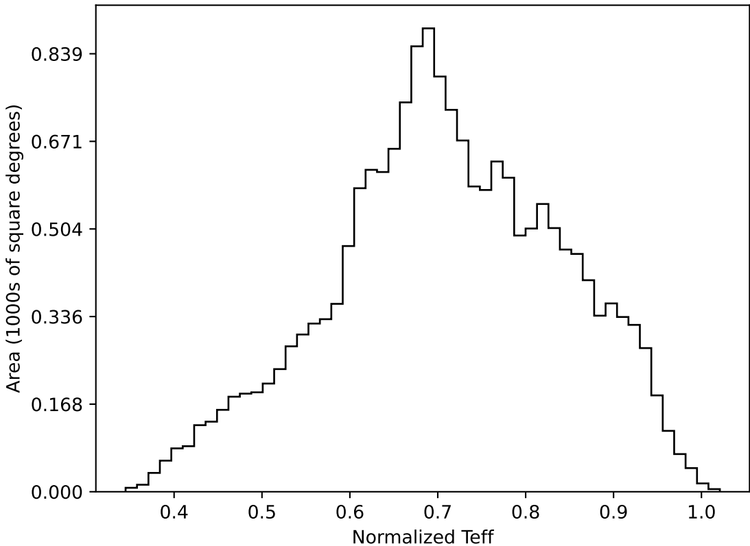
ddf_loaded_half_fl8_v3.4_10yrs WFD all bands: Normalized Teff
