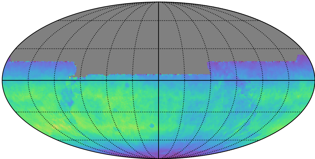
ddf_loaded_half_fl8_v3.4_10yrs All sky y band: Normalized Teff
