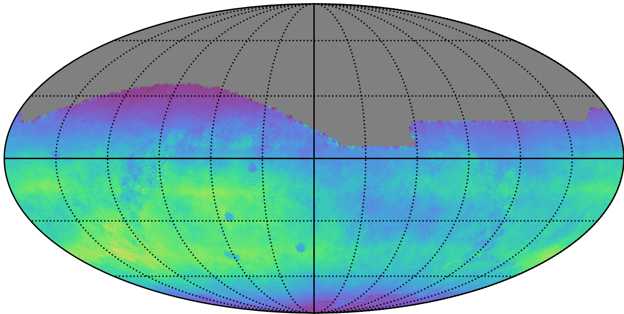
ddf_loaded_half_fl8_v3.4_10yrs All sky r band: Normalized Teff
