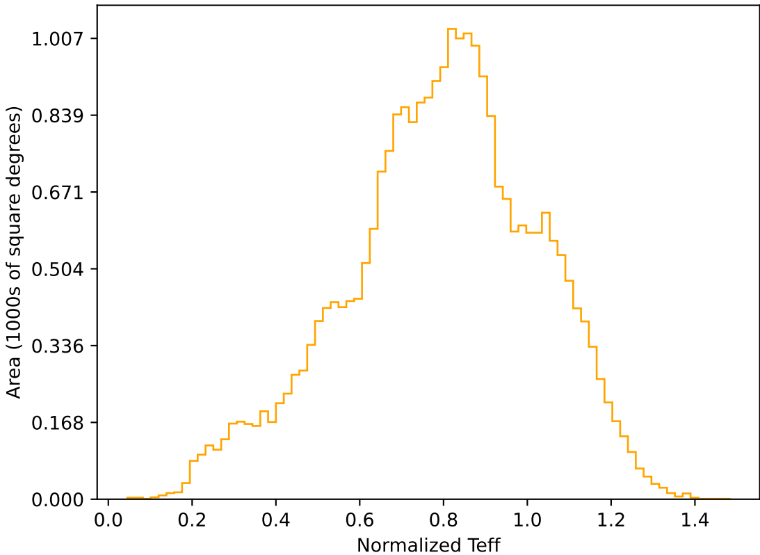
ddf_loaded_half_fl8_v3.4_10yrs All sky r band: Normalized Teff
