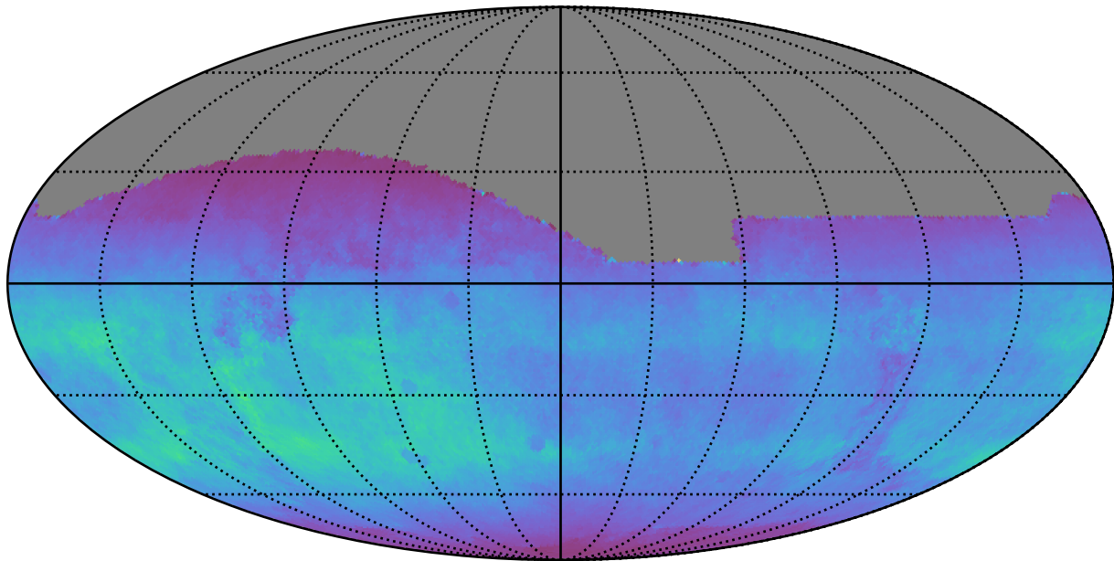
ddf_loaded_half_fl8_v3.4_10yrs All sky i band: Normalized Teff
