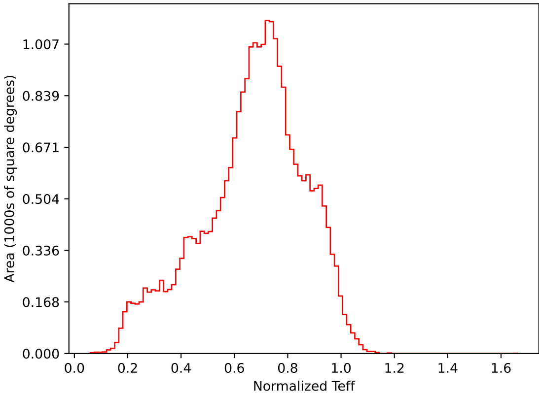
ddf_loaded_half_fl8_v3.4_10yrs All sky i band: Normalized Teff
