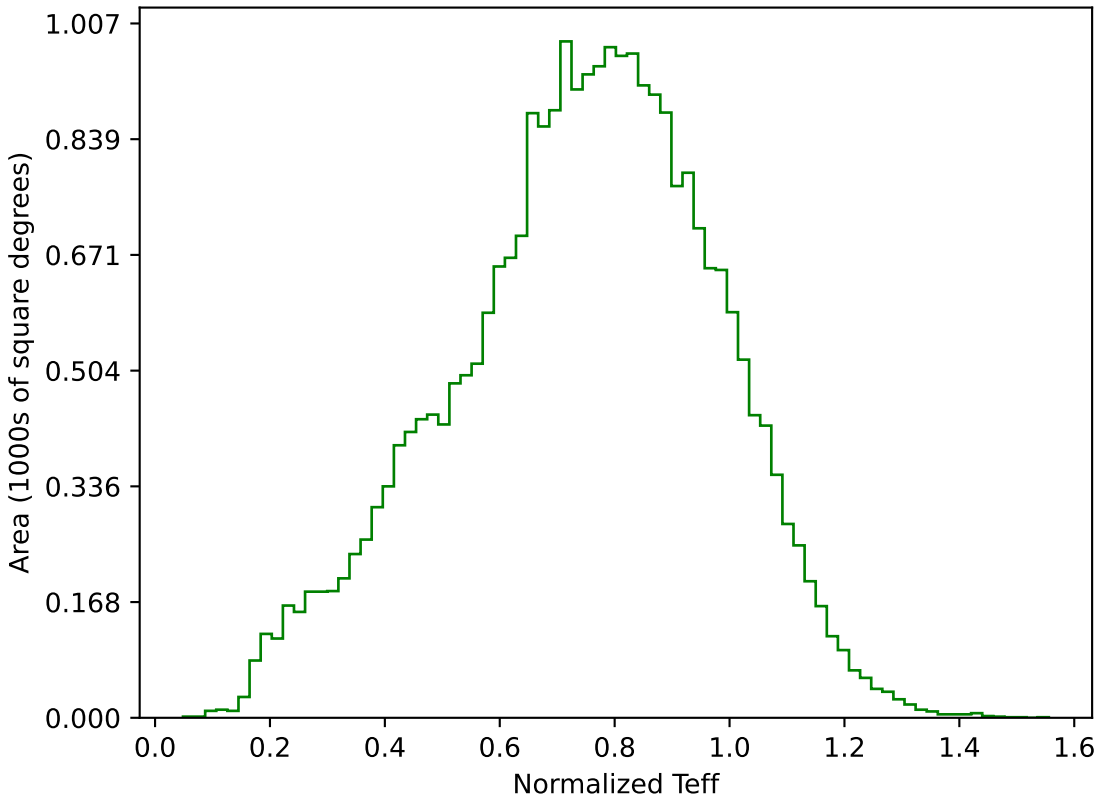
ddf_loaded_half_fl8_v3.4_10yrs All sky g band: Normalized Teff
