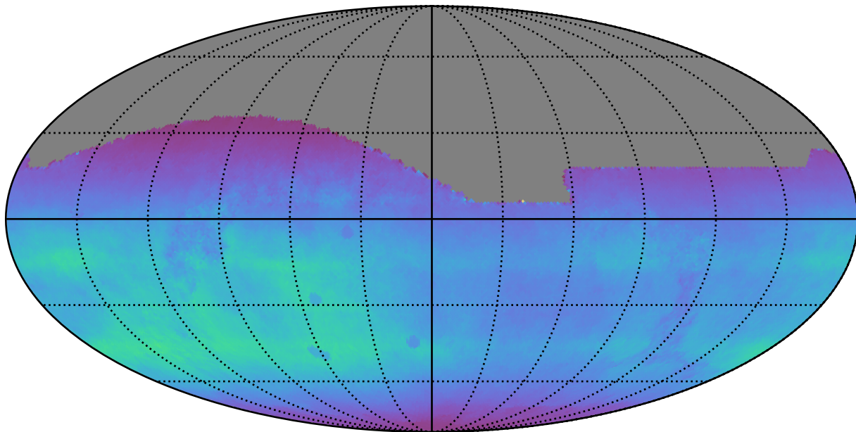
ddf_loaded_half_fl8_v3.4_10yrs All sky all bands: Normalized Teff
