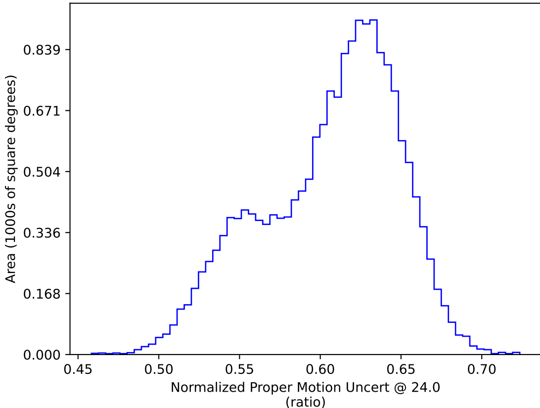
ddf_loaded_half_fl8_v3.4_10yrs WFD: Normalized Proper Motion Uncert @ 24.0
