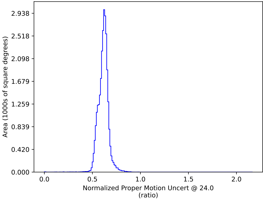
ddf_loaded_half_fl8_v3.4_10yrs All sky: Normalized Proper Motion Uncert @ 24.0
