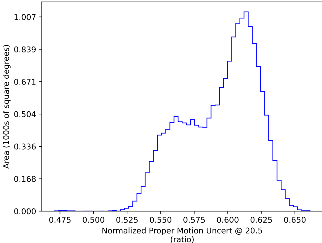
ddf_loaded_half_fl8_v3.4_10yrs WFD: Normalized Proper Motion Uncert @ 20.5
