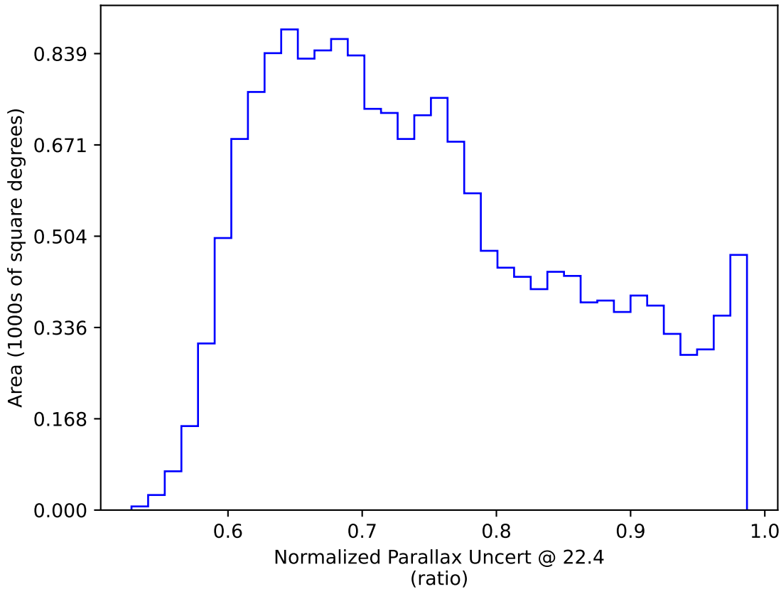
ddf_loaded_half_fl8_v3.4_10yrs WFD: Normalized Parallax Uncert @ 22.4
