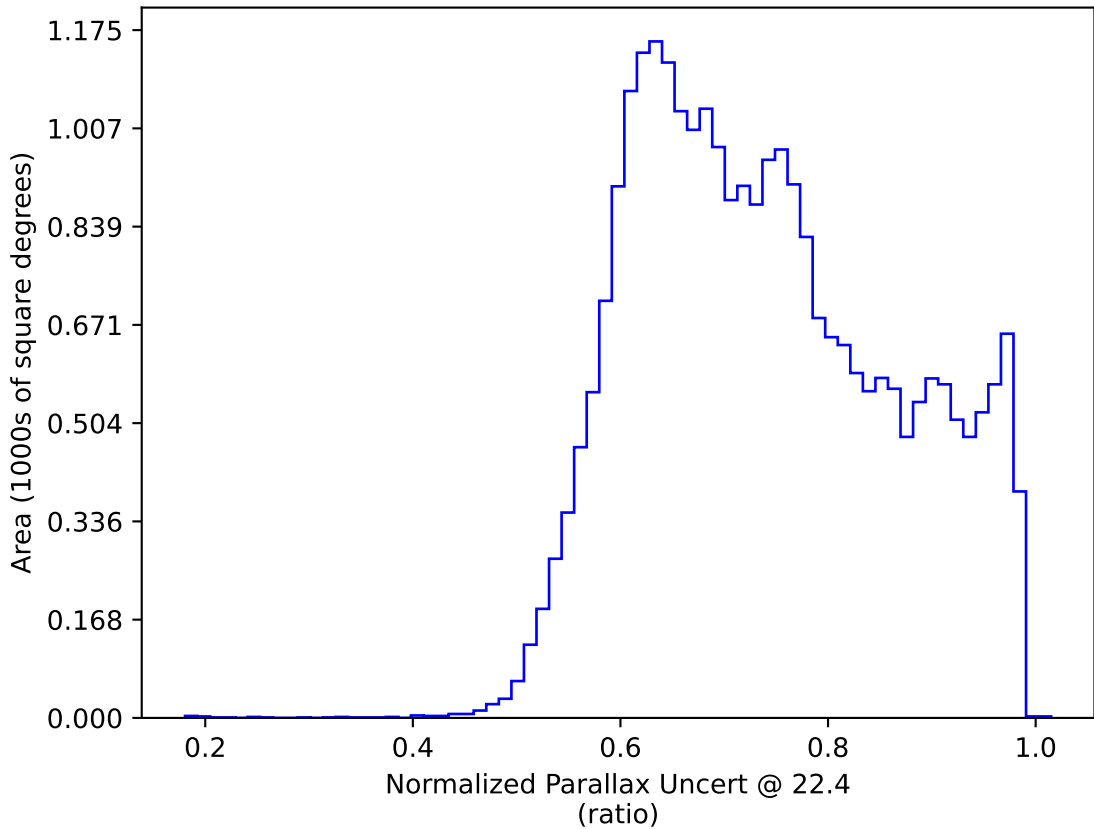
ddf_loaded_half_fl8_v3.4_10yrs All sky: Normalized Parallax Uncert @ 22.4
