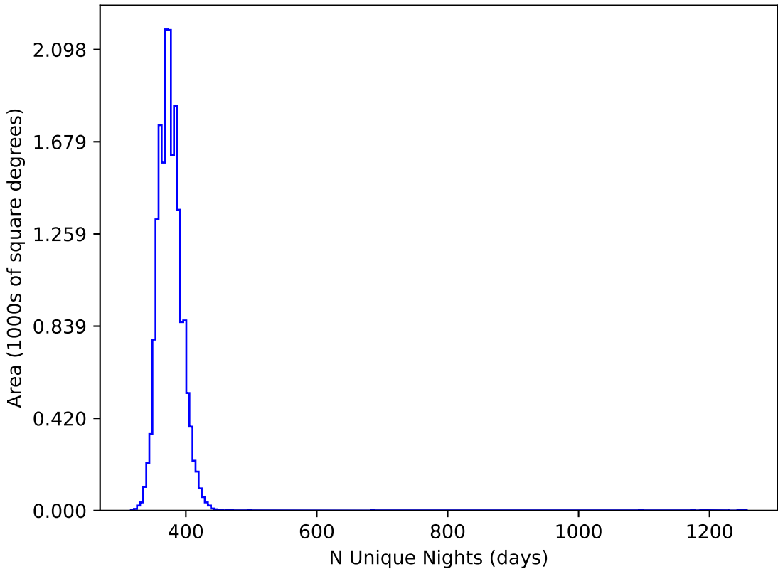
ddf_loaded_half_fl8_v3.4_10yrs WFD all bands: N Unique Nights
