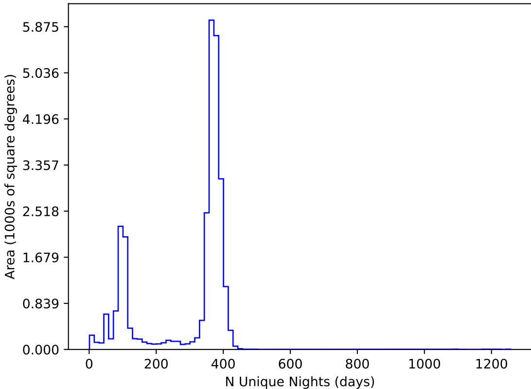
ddf_loaded_half_fl8_v3.4_10yrs All sky all bands: N Unique Nights
