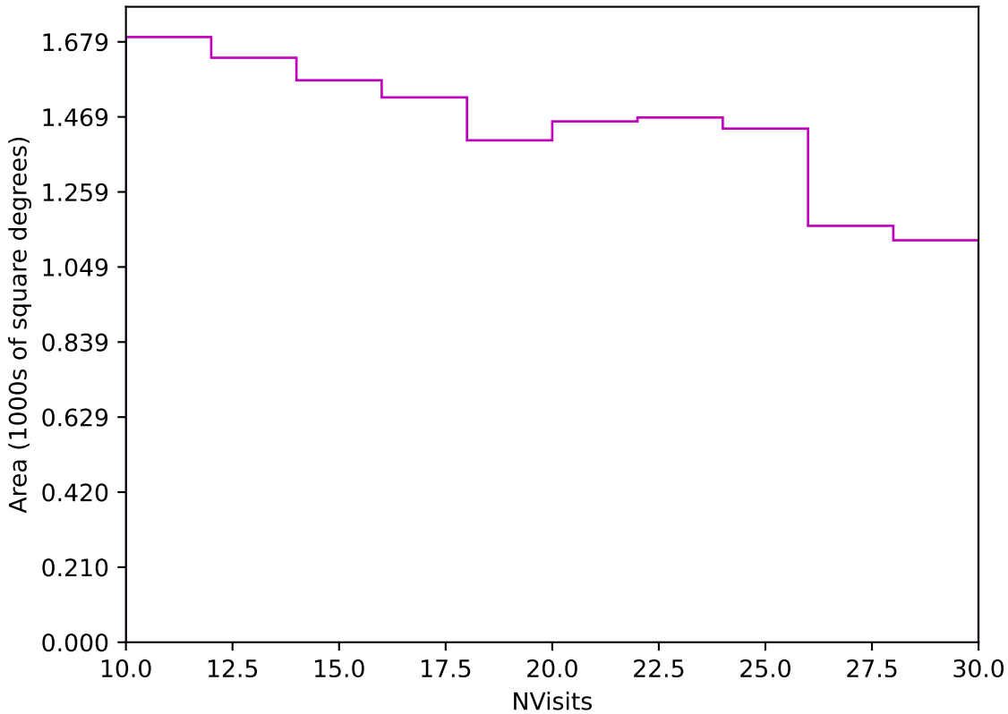
ddf_loaded_half_fl8_v3.4_10yrs Yr 3-4 z band: NVisits
