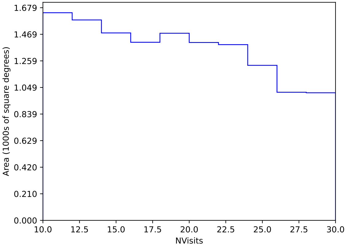
ddf_loaded_half_fl8_v3.4_10yrs Yr 3-4 y band: NVisits
