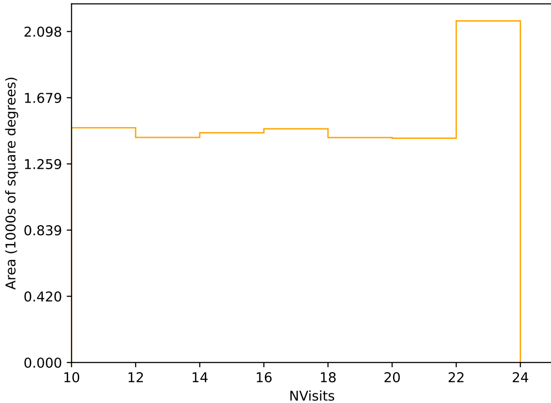
ddf_loaded_half_fl8_v3.4_10yrs Yr 3-4 r band: NVisits
