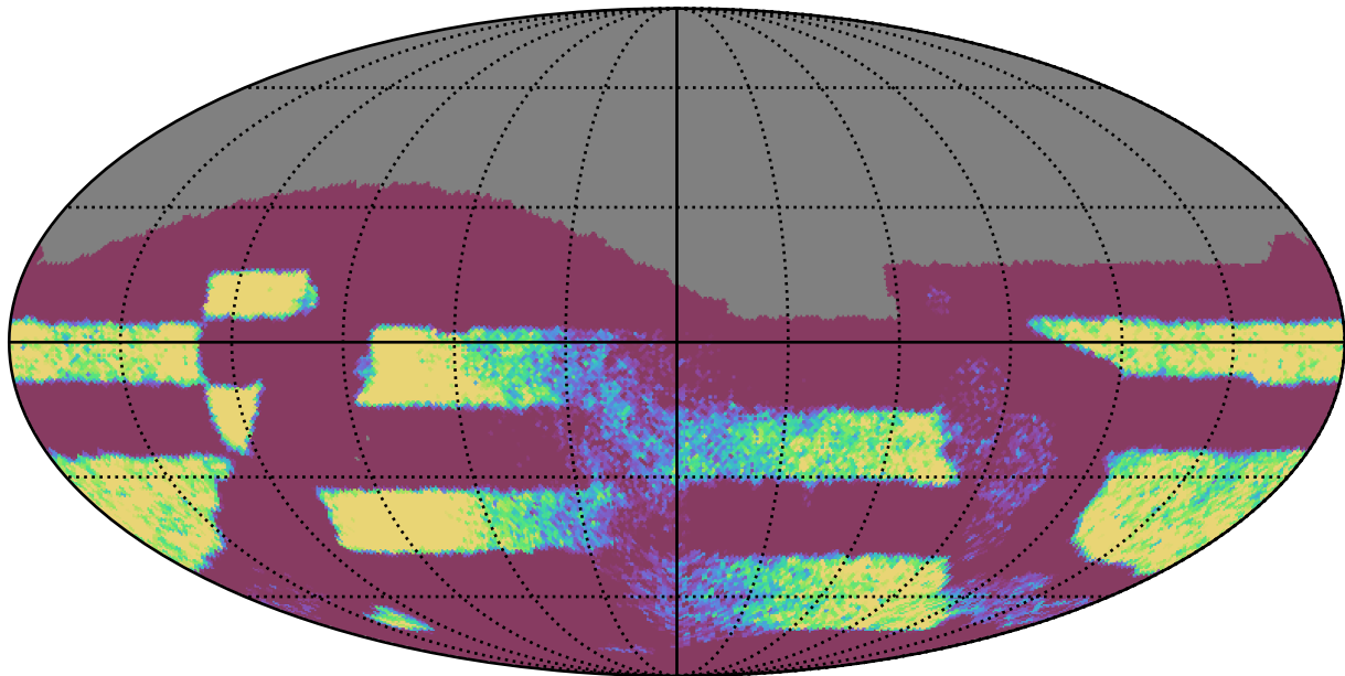
ddf_loaded_half_fl8_v3.4_10yrs Yr 3-4 all bands: NVisits
