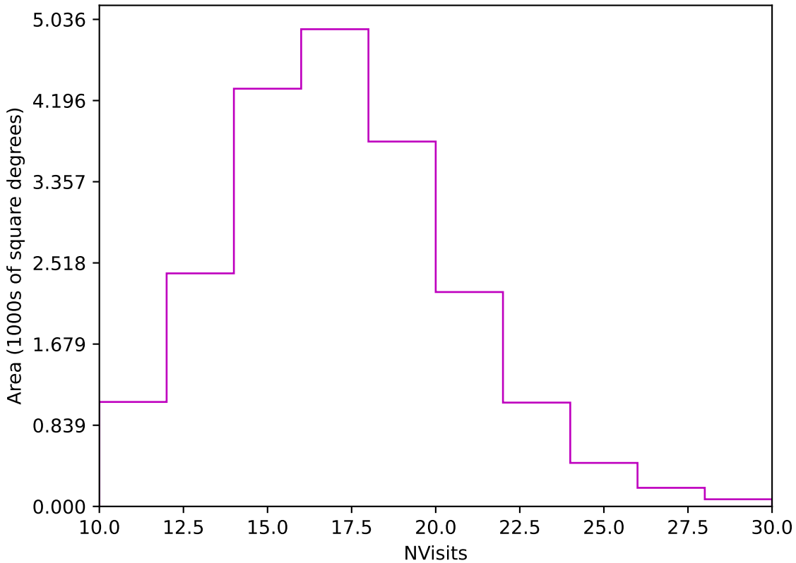
ddf_loaded_half_fl8_v3.4_10yrs Yr 1 z band: NVisits
