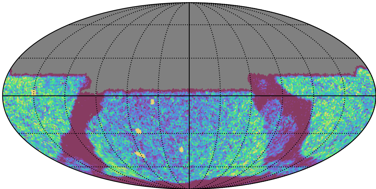
ddf_loaded_half_fl8_v3.4_10yrs Yr 1 y band: NVisits
