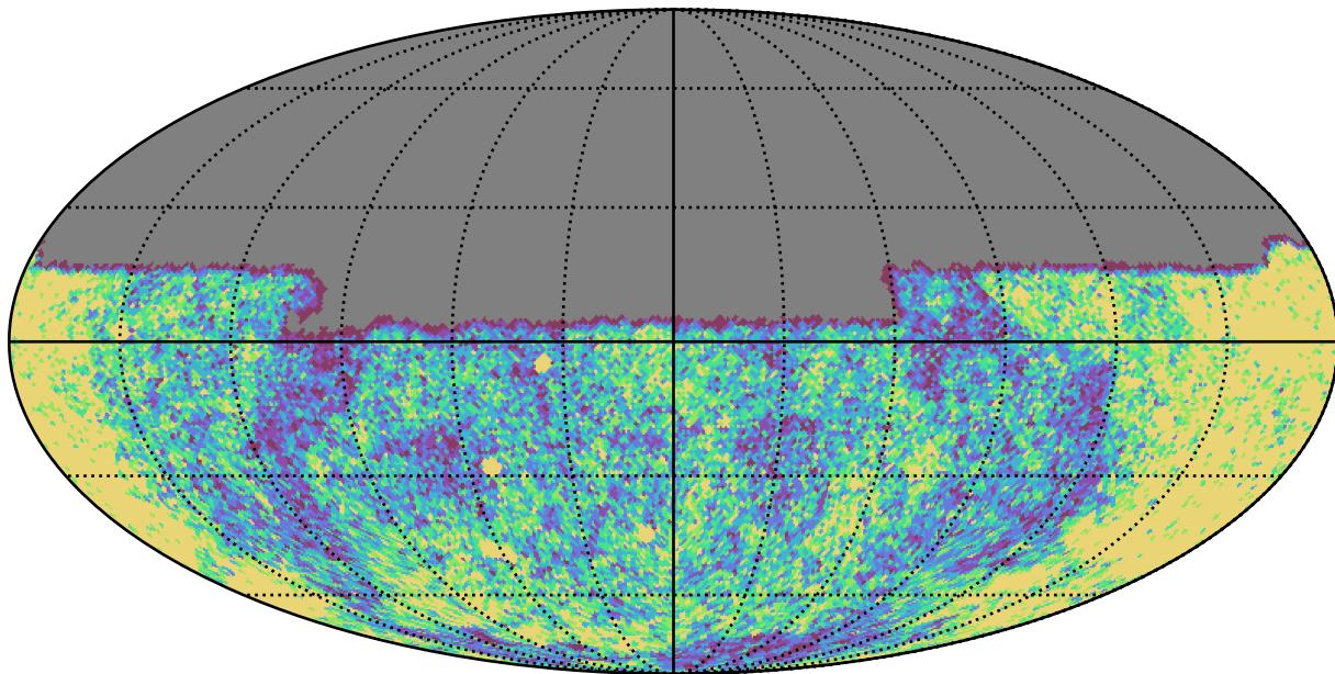
ddf_loaded_half_fl8_v3.4_10yrs Yr 1 u band: NVisits
