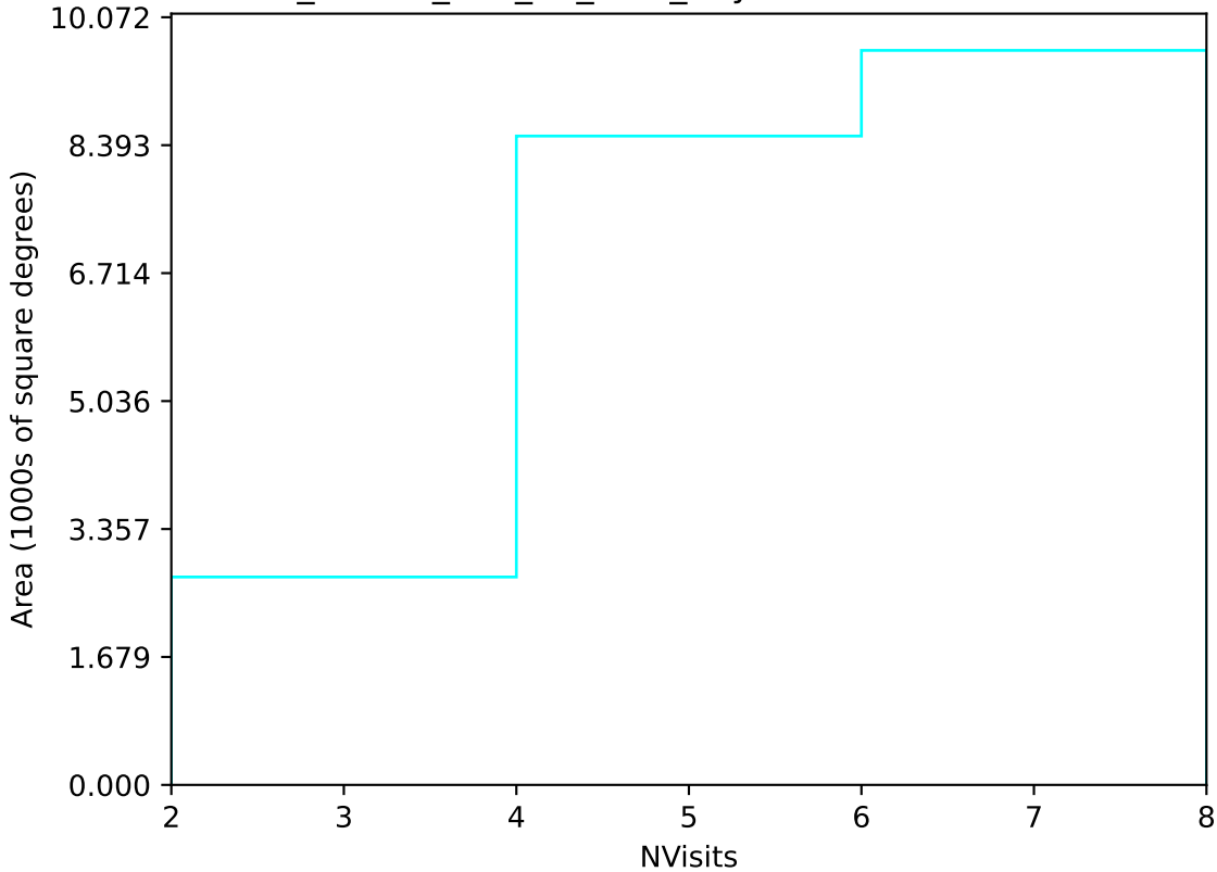
ddf_loaded_half_fl8_v3.4_10yrs Yr 1 u band: NVisits
