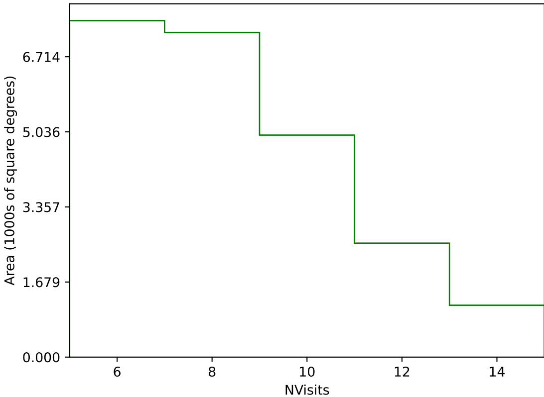
ddf_loaded_half_fl8_v3.4_10yrs Yr 1 g band: NVisits
