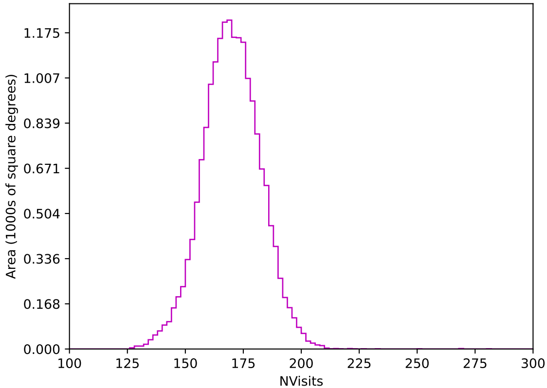
ddf_loaded_half_fl8_v3.4_10yrs WFD z band: NVisits
