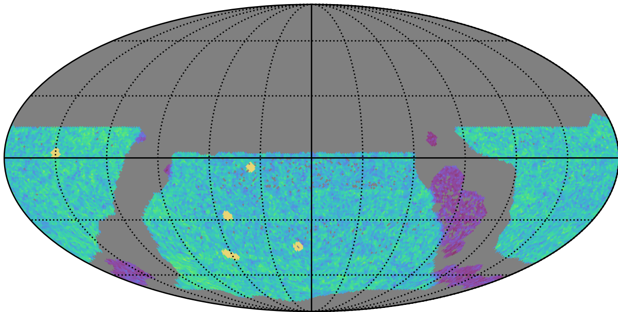
ddf_loaded_half_fl8_v3.4_10yrs WFD u band: NVisits
