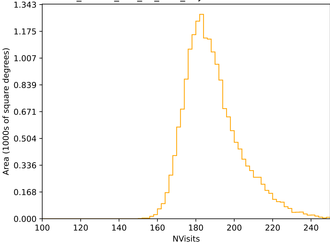
ddf_loaded_half_fl8_v3.4_10yrs WFD r band: NVisits
