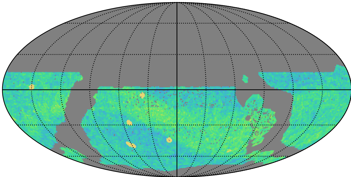
ddf_loaded_half_fl8_v3.4_10yrs WFD i band: NVisits
