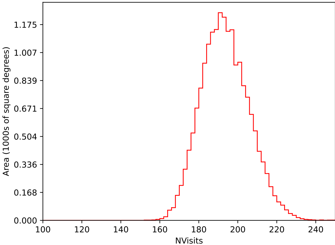
ddf_loaded_half_fl8_v3.4_10yrs WFD i band: NVisits
