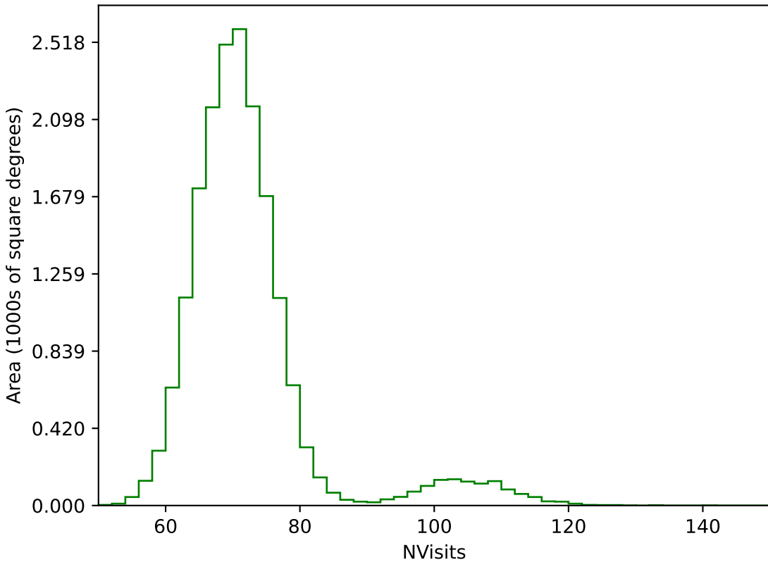
ddf_loaded_half_fl8_v3.4_10yrs WFD g band: NVisits
