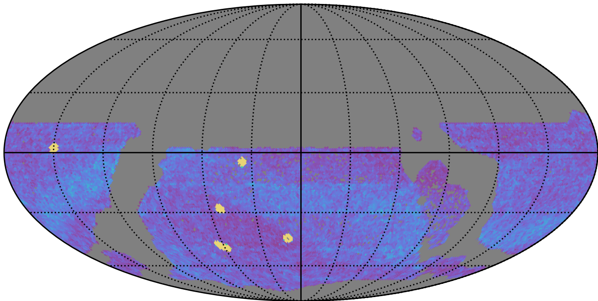
ddf_loaded_half_fl8_v3.4_10yrs WFD all bands: NVisits
